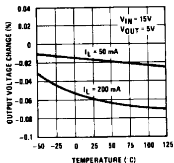
Output Voltage Change with Temperature (Normalized)
