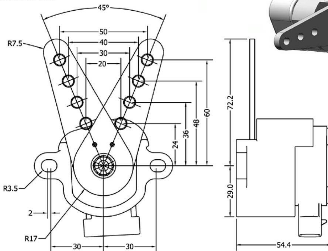
Dimensions [mm]
