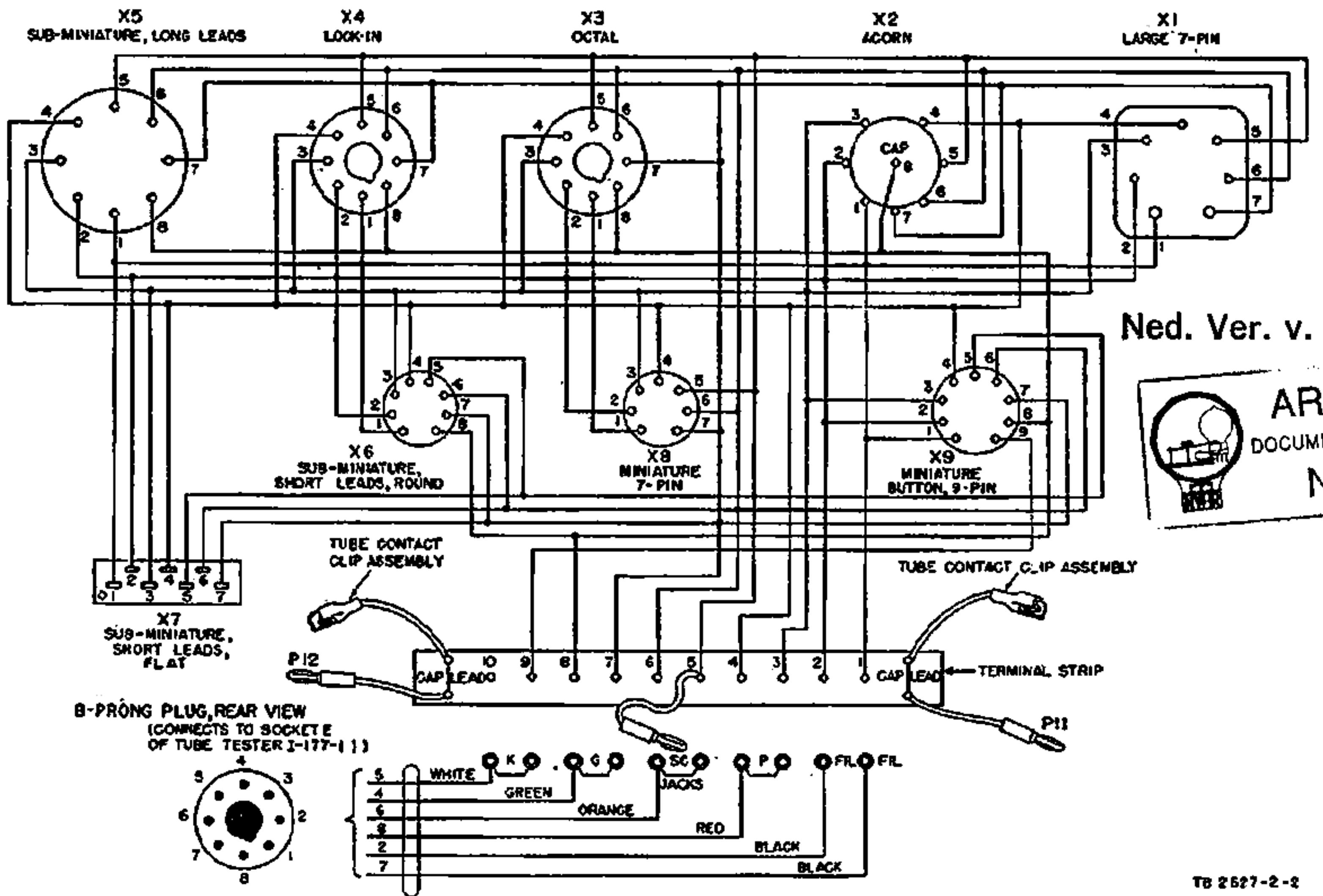
Figure 2. Tube Socket Adapter Kit MX-949/U, wiring diagram.
