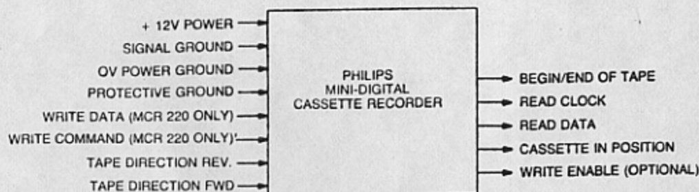
Fig. 6. Mini-DCR - Interface Diagram.
