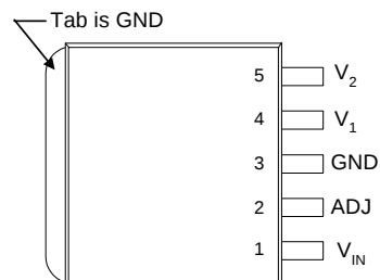
DF PACKAGE (Top View)
