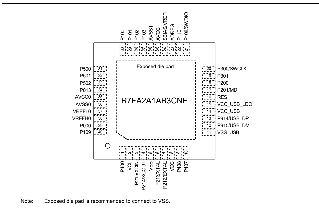
Figure 1.5 Pin assignment for QFN 40-pin
