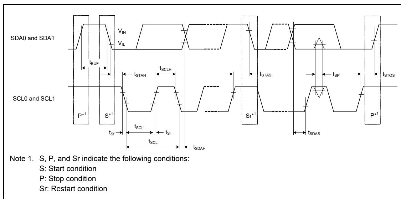
Figure 2.57 I²C bus interface input/output timing
