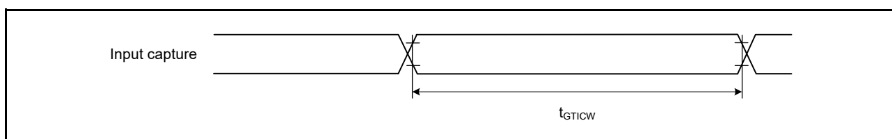
Figure 2.38 GPT input capture timing
