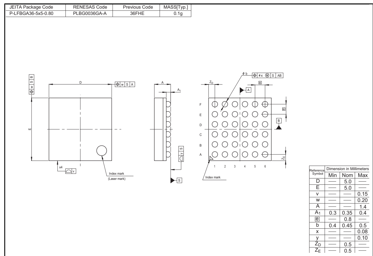
Figure 1.3 BGA 36-pin
