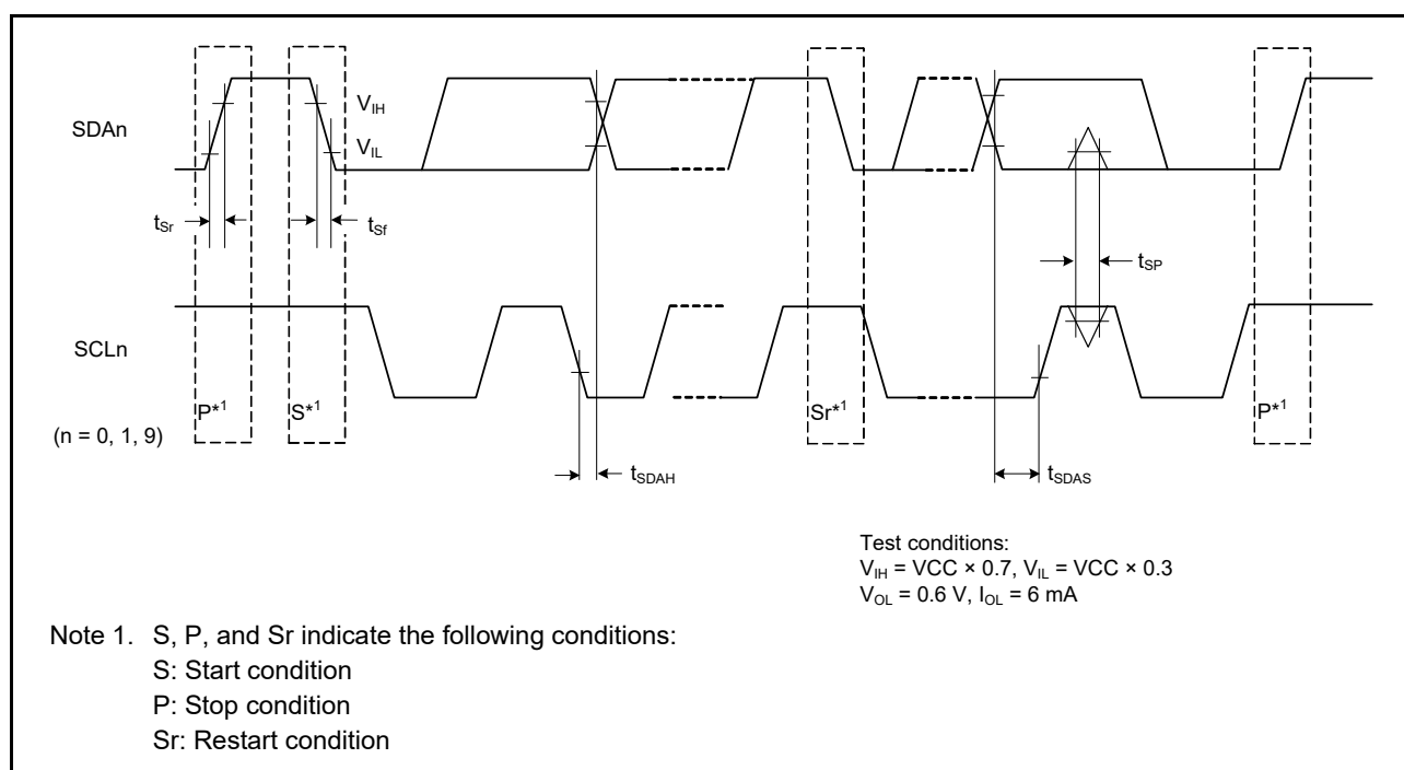
Figure 2.49 SCI simple IIC mode timing
