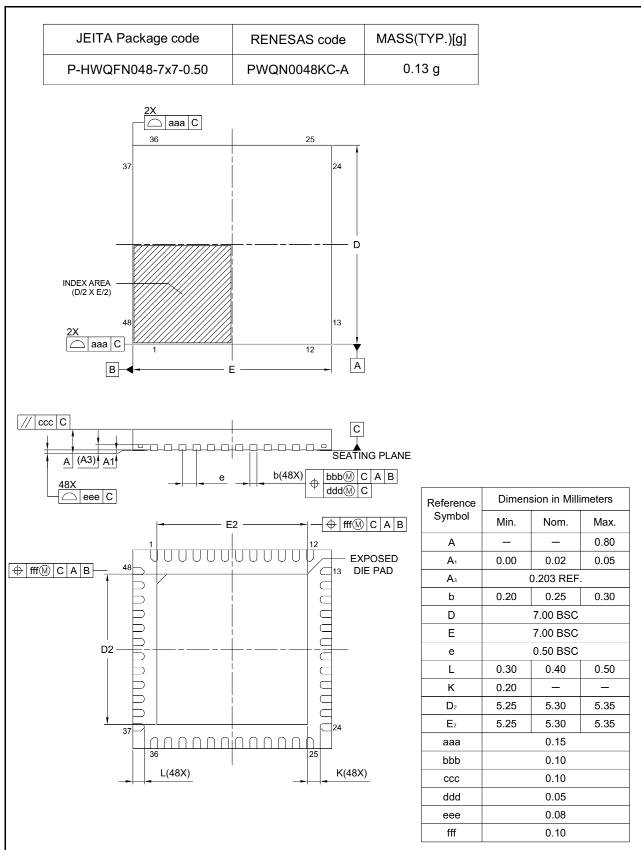
Figure 1.5 QFN 48-pin (2)
