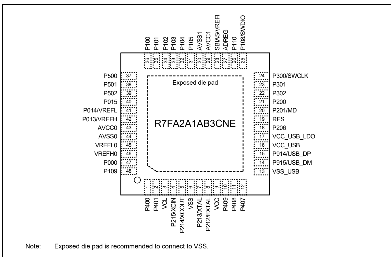
Figure 1.4 Pin assignment for QFN 48-pin
