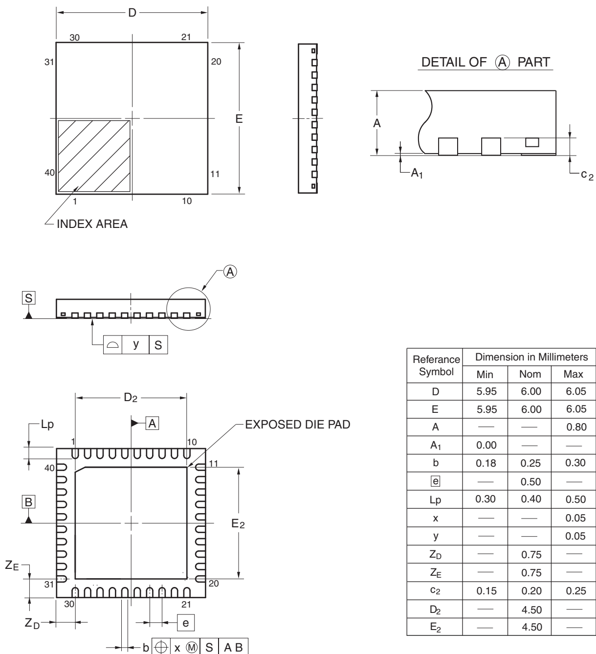
Figure 1.6 QFN 40-pin (1)
