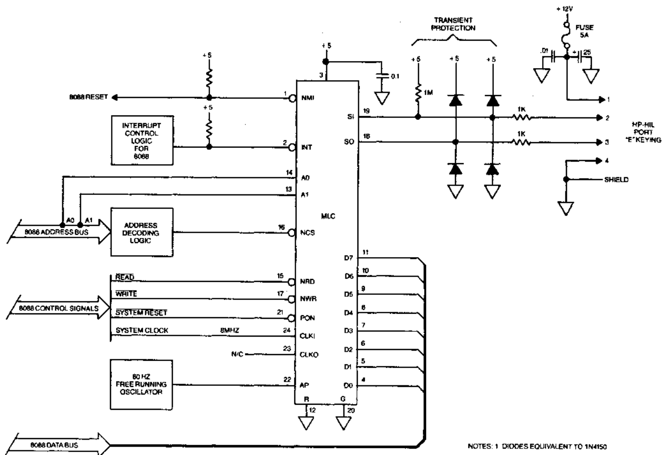
Figure 3-2. Example MLC Interface
