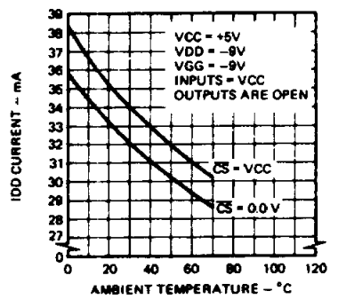
IDD Current Versus Temperature
