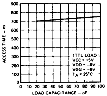
Access Time Versus Load Capacitance
