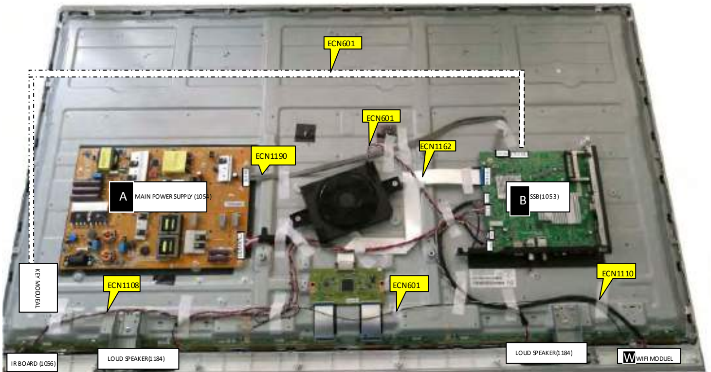
Cable dressing (49" 6482 series)
