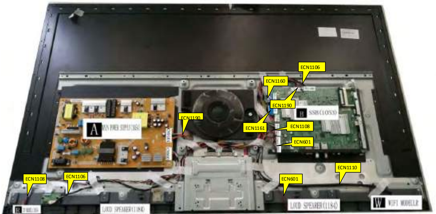
Cable dressing (49"/55"/65" 7502 series)
