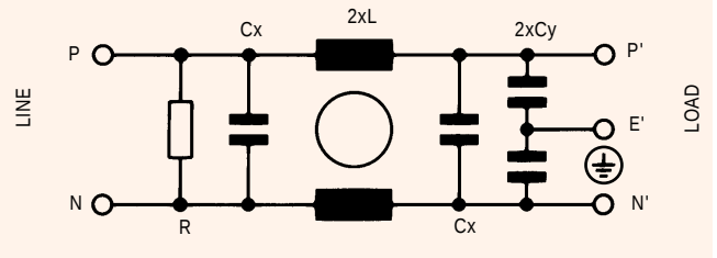
FN 401 (1.5A)
