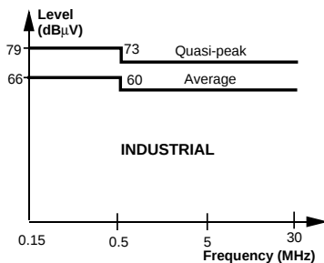
Figure 2. EN 50081-2 limits
