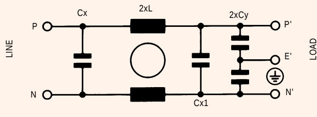
FN 401 (0.8A)
