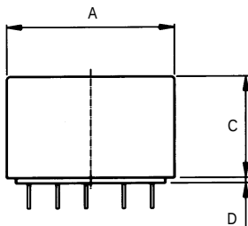
Housing A6
