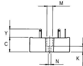
Housing KB2
