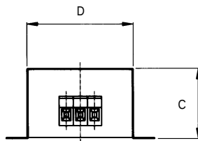
Housing B7, B8, B11 (Connection /29)
