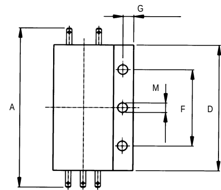
Housing A7B
