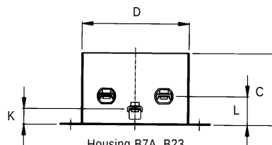
Housing B7A, B23 (Connection /03)
