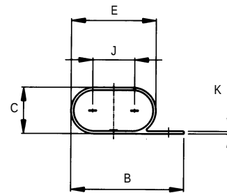
Housing A7B
