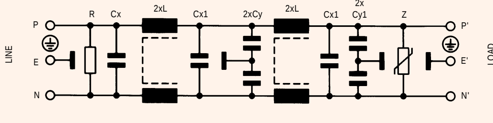
FN 352Z-6
