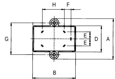
Housing KB2
