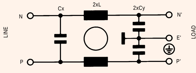
FN 332
