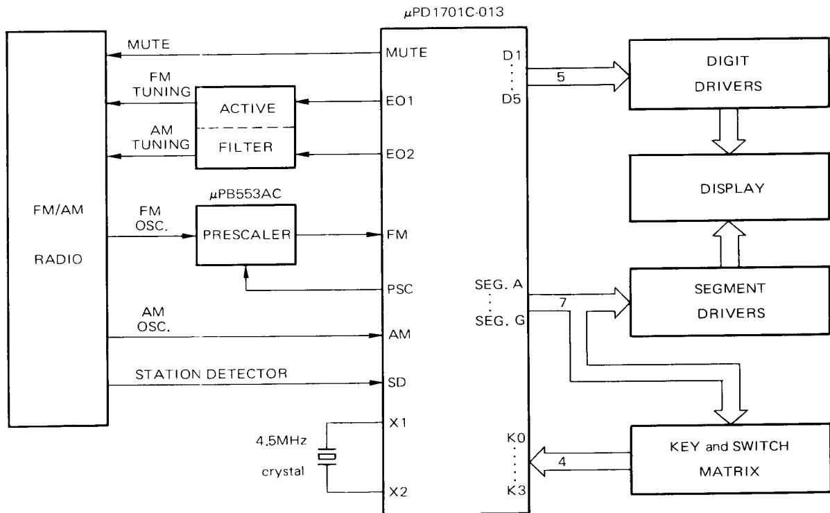
Fig. 1 Block Diagram
