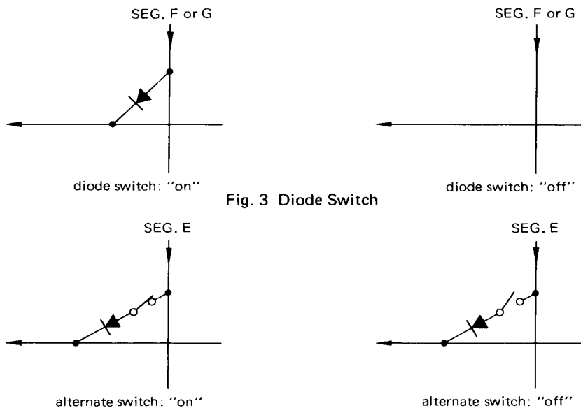
Fig. 4 Alternate Switch
