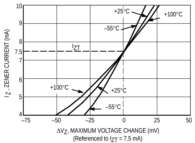
Figure 3. 1N821A Series
