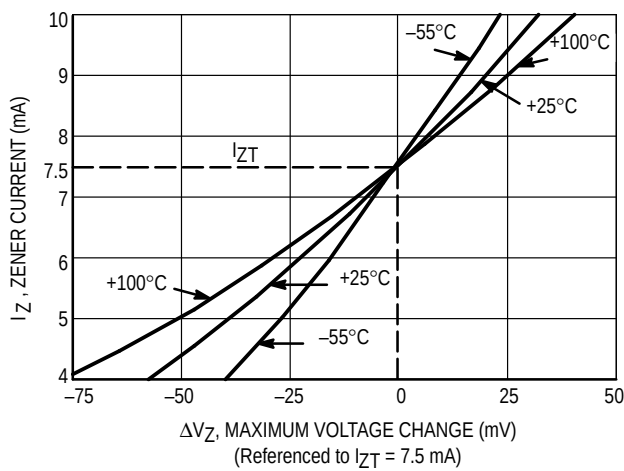
Figure 2. 1N821 Series
