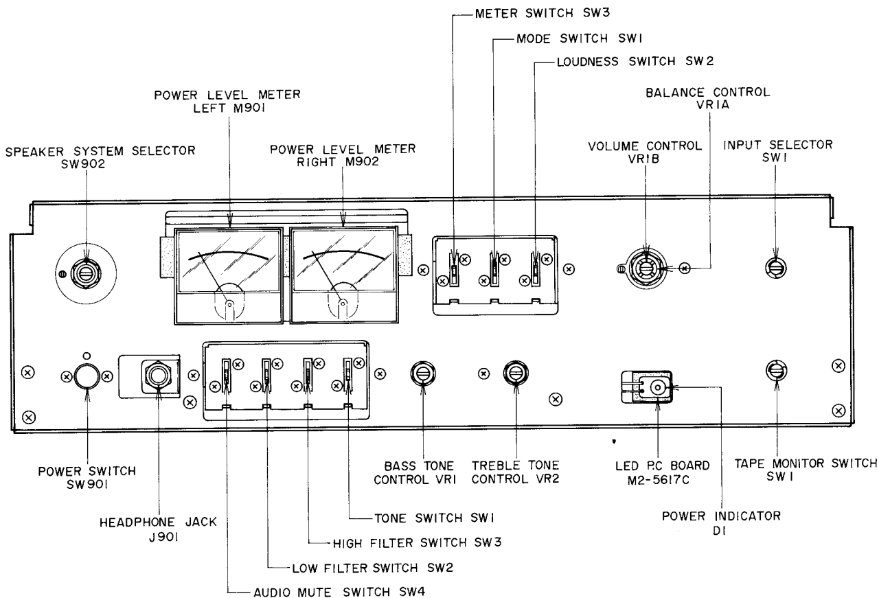
Fig. 3 Front View
