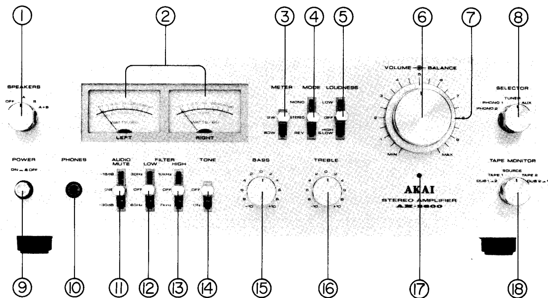
Fig. 1 Controls
