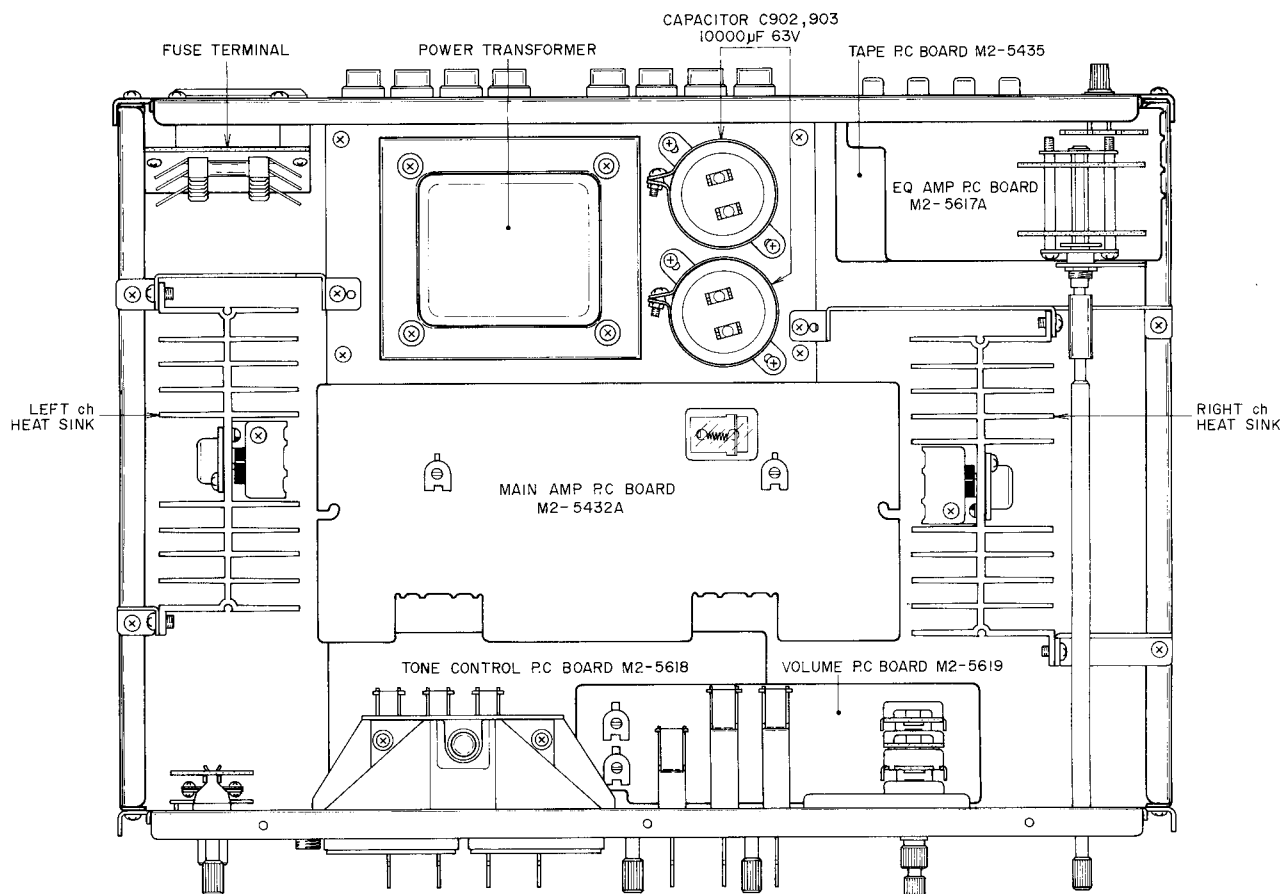
Fig. 2 Top View
