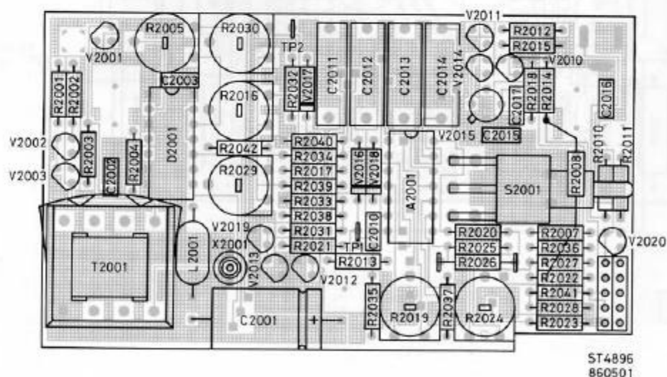
Figure 8.3 Illumination pcb N2 -mAs conductor side PM2618/32
