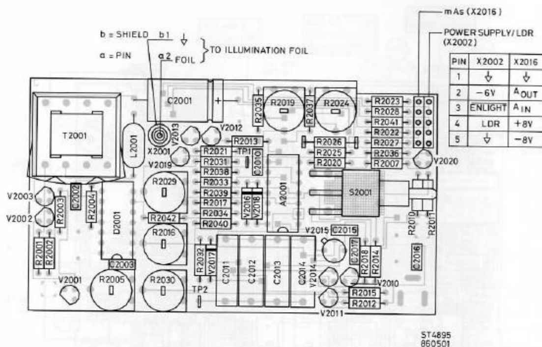
Illumination pcb N2 -mAs component side PM2618/32
