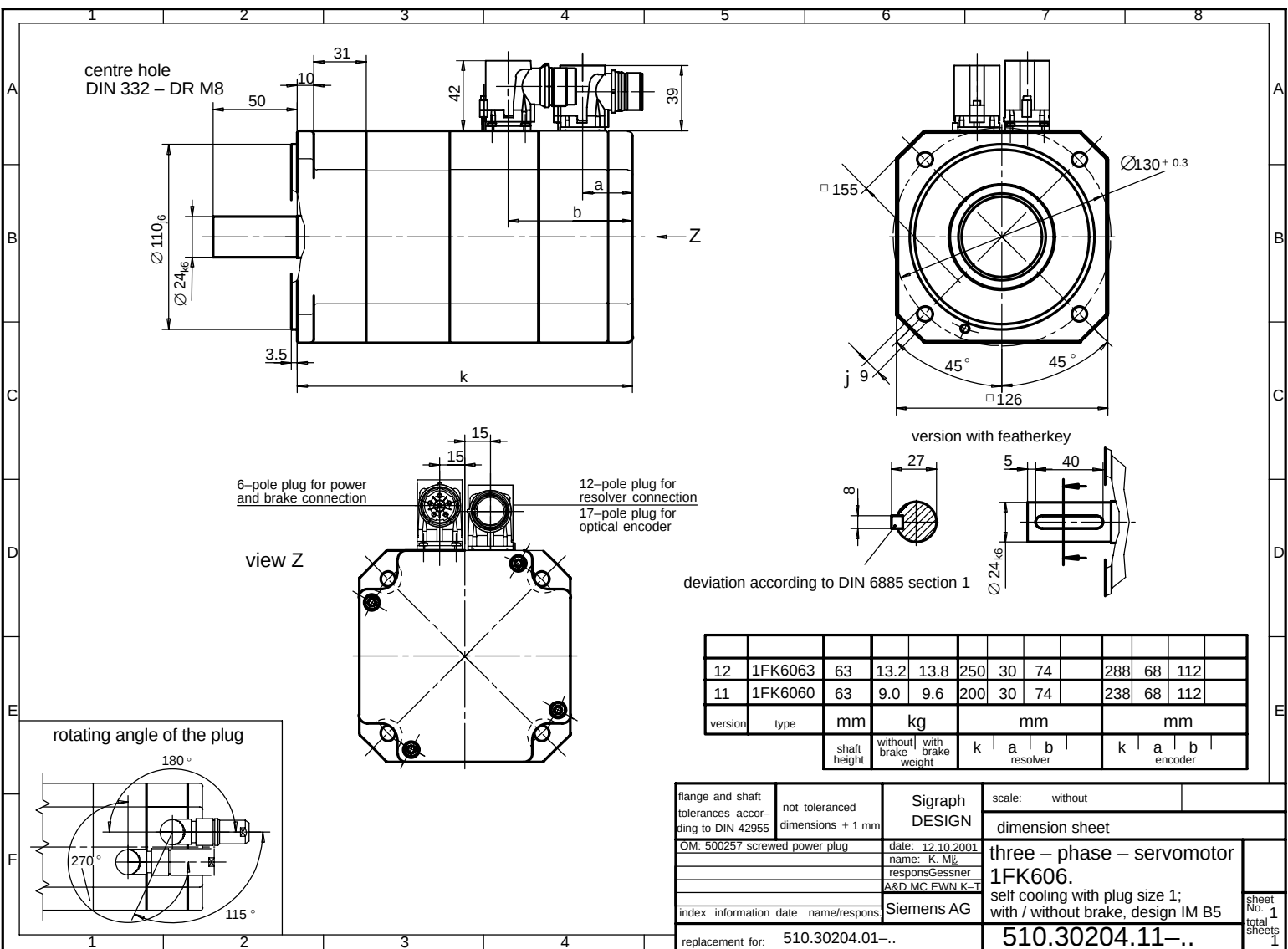
Fig. 4-3 1FK6060 standard, non-ventilated with angled connector, Size 1
