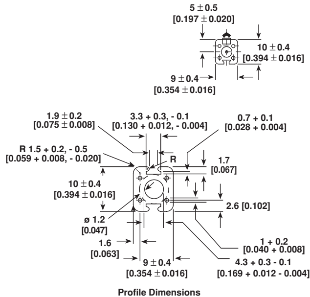
Profile Dimensions
