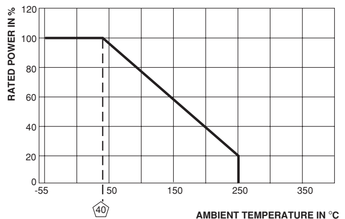
Derating KKE..Si
