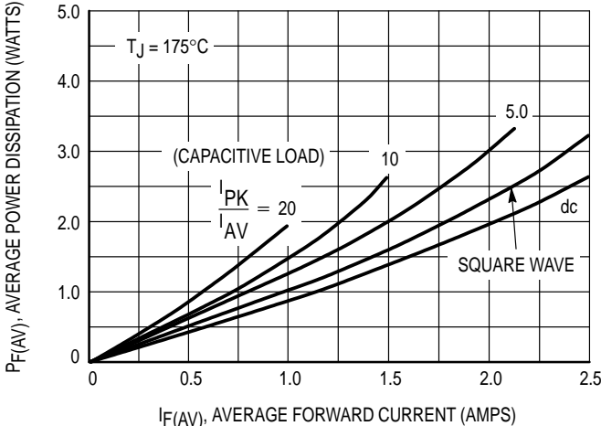
Figure 9. Power Dissipation
