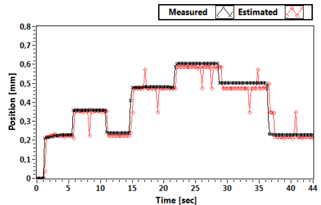
Figure 15. Open loop position estimation.
