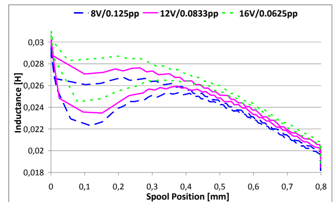
Figure 11. Inductance at different supply voltages.
