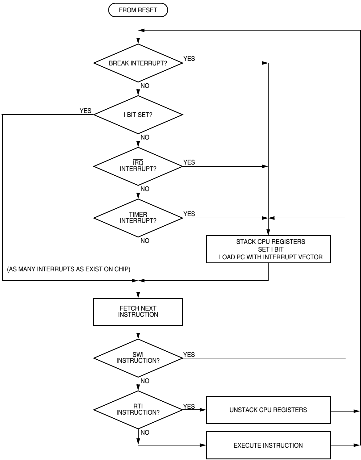
Figure 14-7. Interrupt Processing
