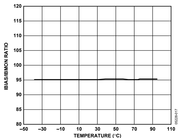
Figure 16. I_{BIAS}/I_{BMON} Gain vs. Temperature, I_{BIAS} = 20\text{mA}
