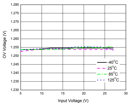
Figure 14. OV Voltage vs. Input Voltage
